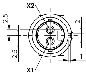
VIEW / VISTA X SCALE / ESCALA 1 : 1
