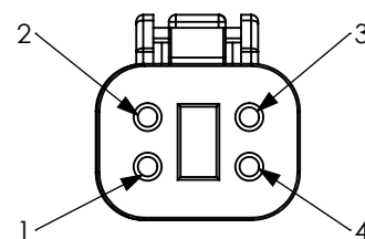
VIEW/VISTA A
