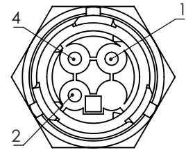
VIEW/VISTA B
