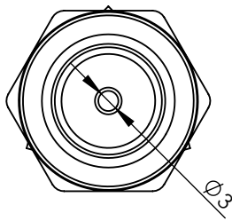
VIEW/VISTA A
