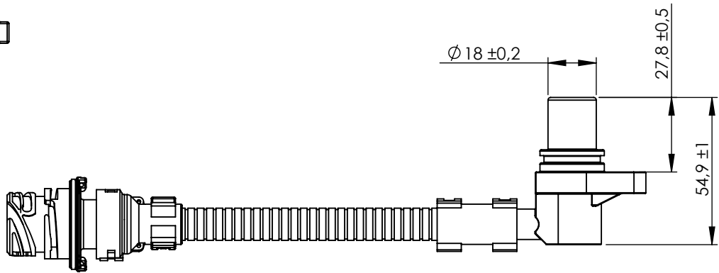
VIEW/VISTA A
