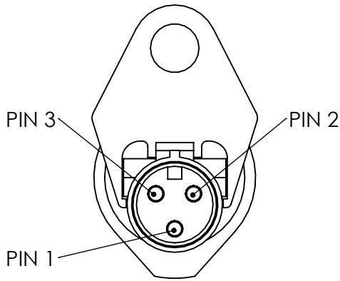
VIEW/VISTA A
