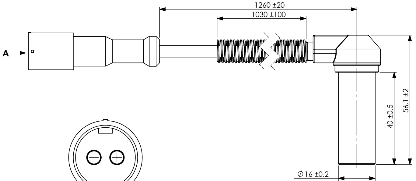
VIEW/VISTA A
