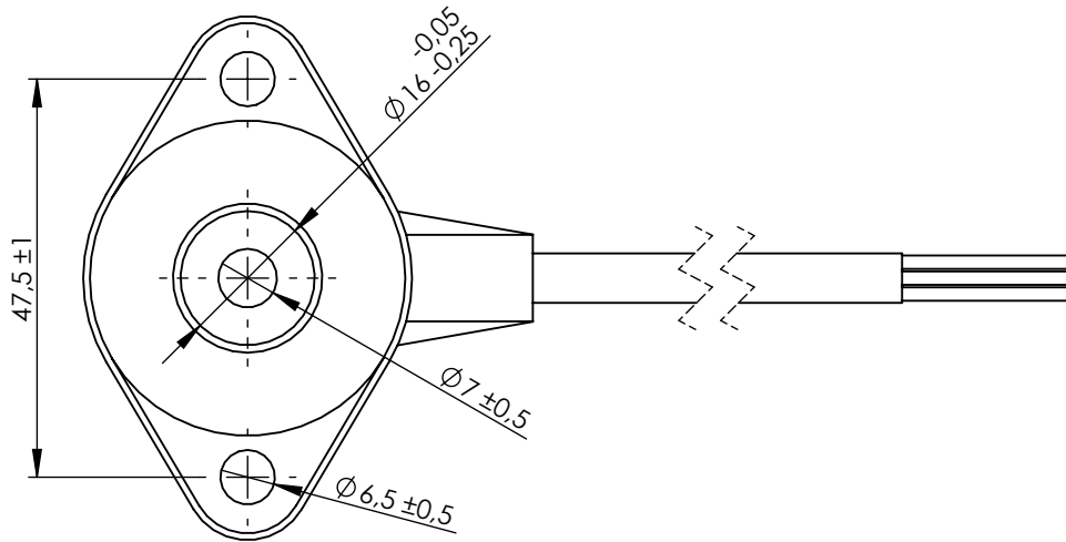
VIEW/VISTA A
