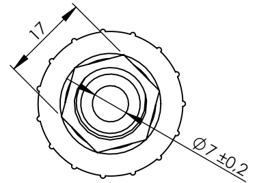
VIEW/VISTA B
