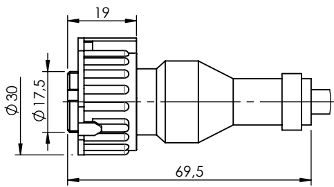
DETAIL / DETALLE X SCALE / ESCALA 2 : 3
