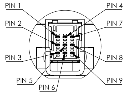
DETAIL/DETALLE A
