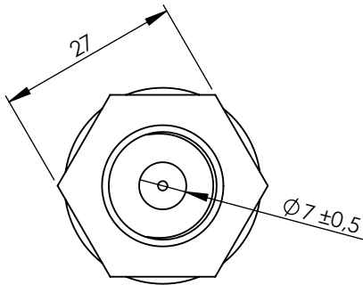
VIEW/VISTA B
