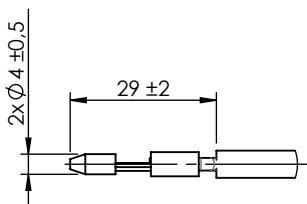
DETAIL / DETALLE X SCALE / ESCALA 2 : 3
