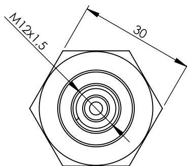
VIEW/VISTA B
