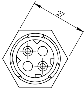
VIEW/VISTA A
